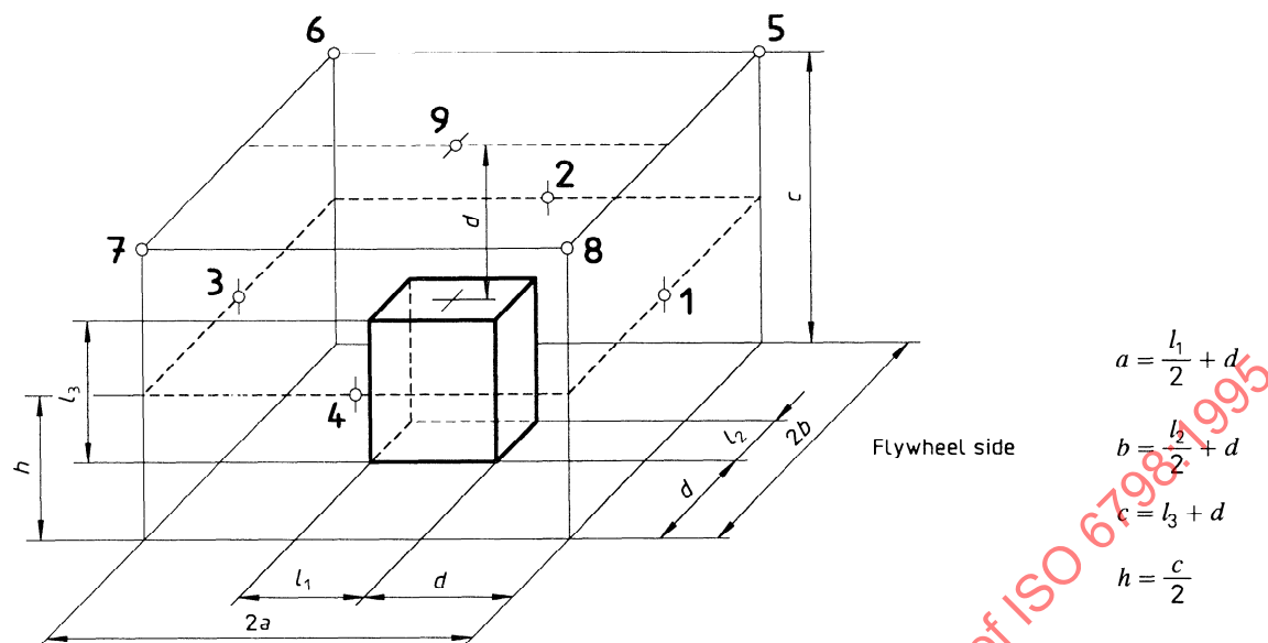
Figure 1 — Arrangement of nine (five) measurement points and measurement surface (For engines with reference parallelepiped dimensions l_1 \leq 2 m, l_2 \leq 2 m, l_3 \leq 2,5 m.)
