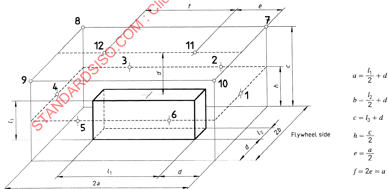
Figure 2 — Arrangement of twelve measurement points and measurement surface (For engines with reference parallelepiped dimensions 2 \text{ m} \leq l_1 < 4 \text{ m} , l_3 \leq 2,5 \text{ m} .)
