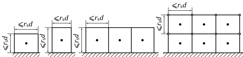
Figure 1 — Microphone positions on the measurement surface
