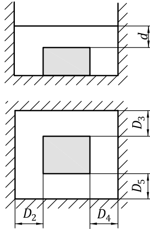
Figure 5 — Five reflecting planes
