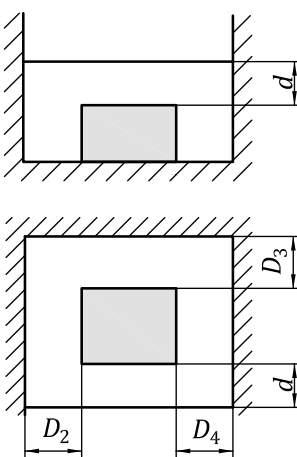
Figure 4 — Four reflecting planes
