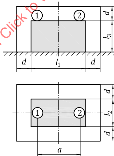
Figure 12 — RSS position for top-up method — Example 1
