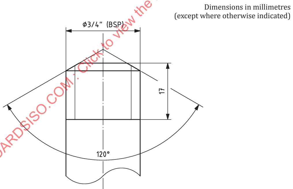
Figure 5 — Mandrel for coupling-nut test
