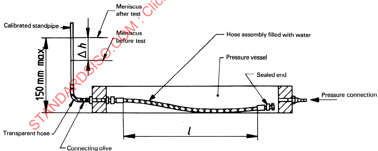
Figure B.1 — Apparatus for determination of resistance to external pressure
