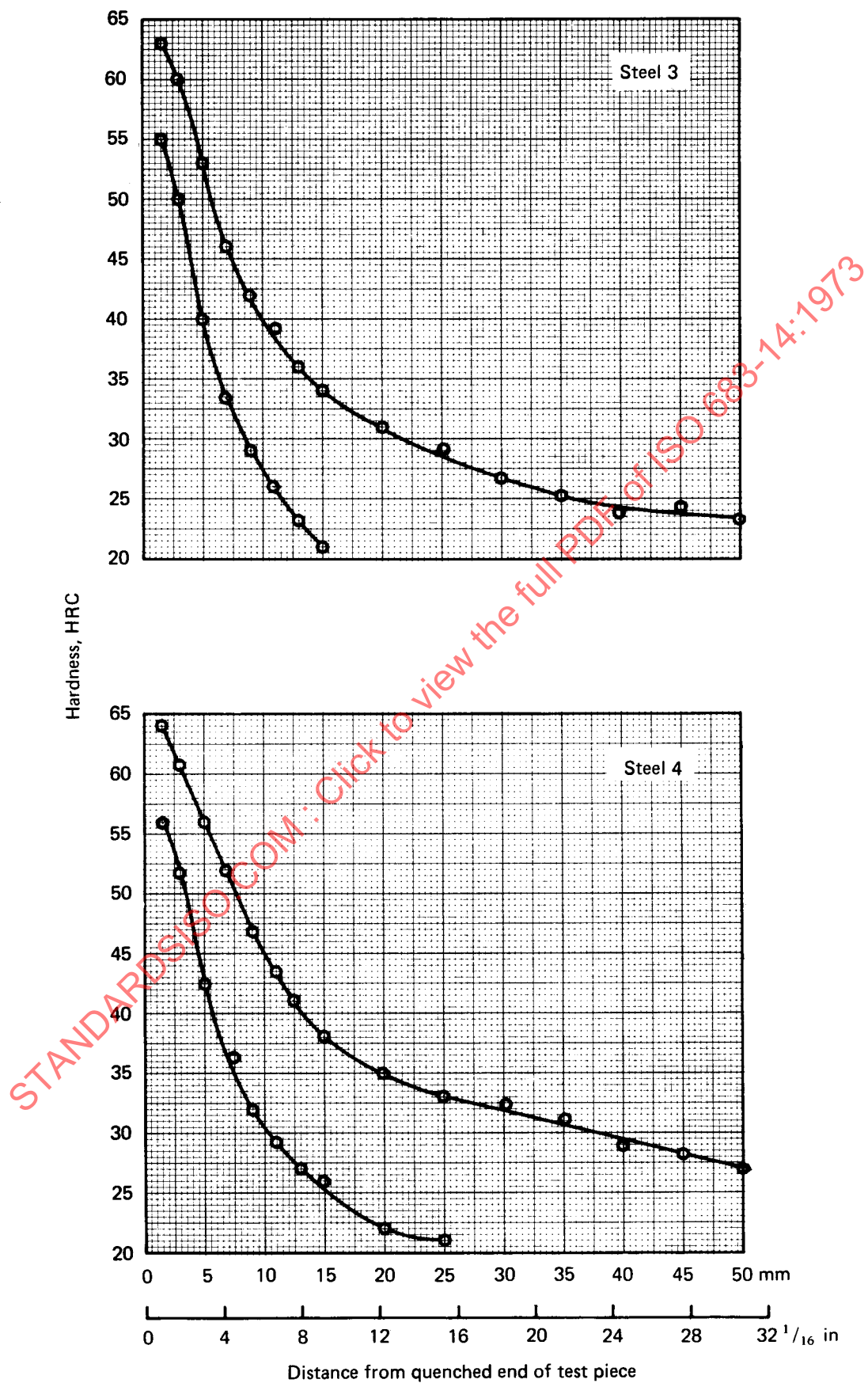
FIGURE 1a – Scatter bands for end-quench hardenability
