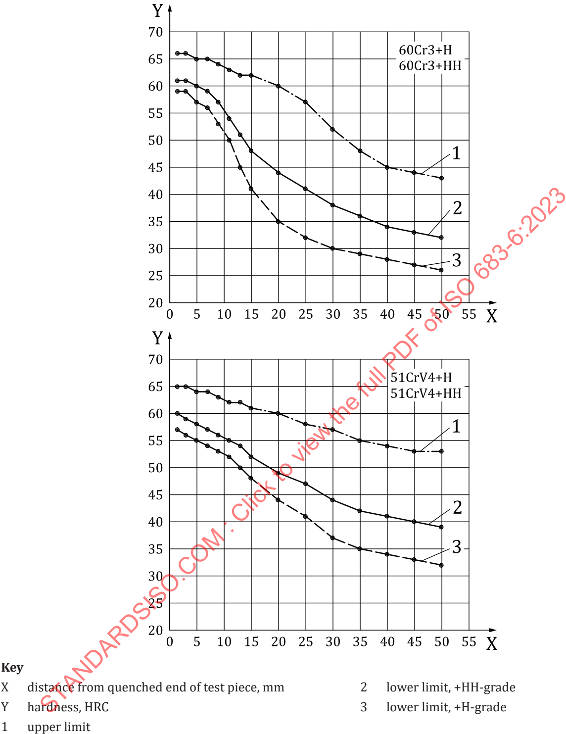
Figure 1 — Scatterbands for end-quench hardenability (continued)
