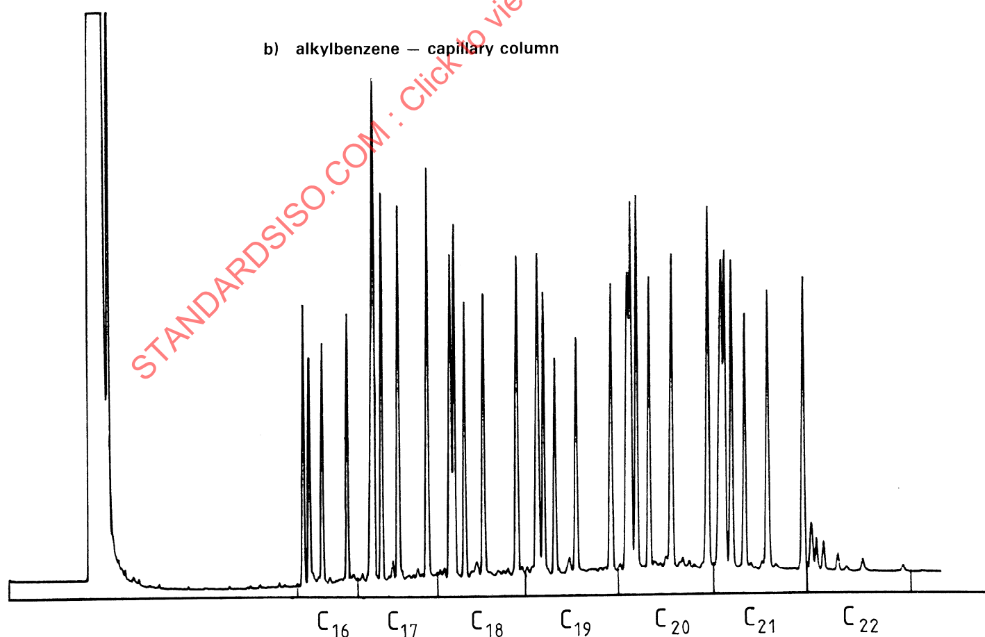
Figure 3 — Typical chromatograms
