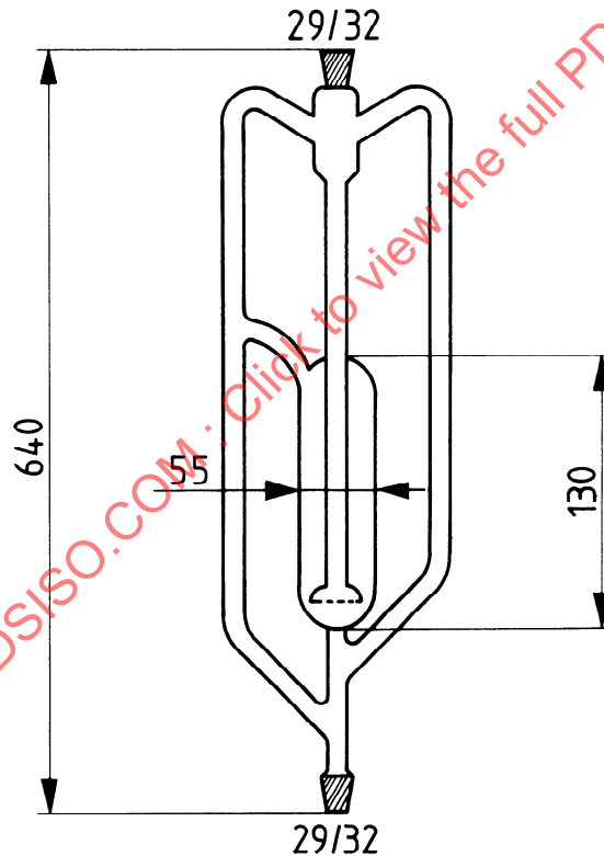
Figure 1 — 300 ml liquid-liquid extractor (6.1)
