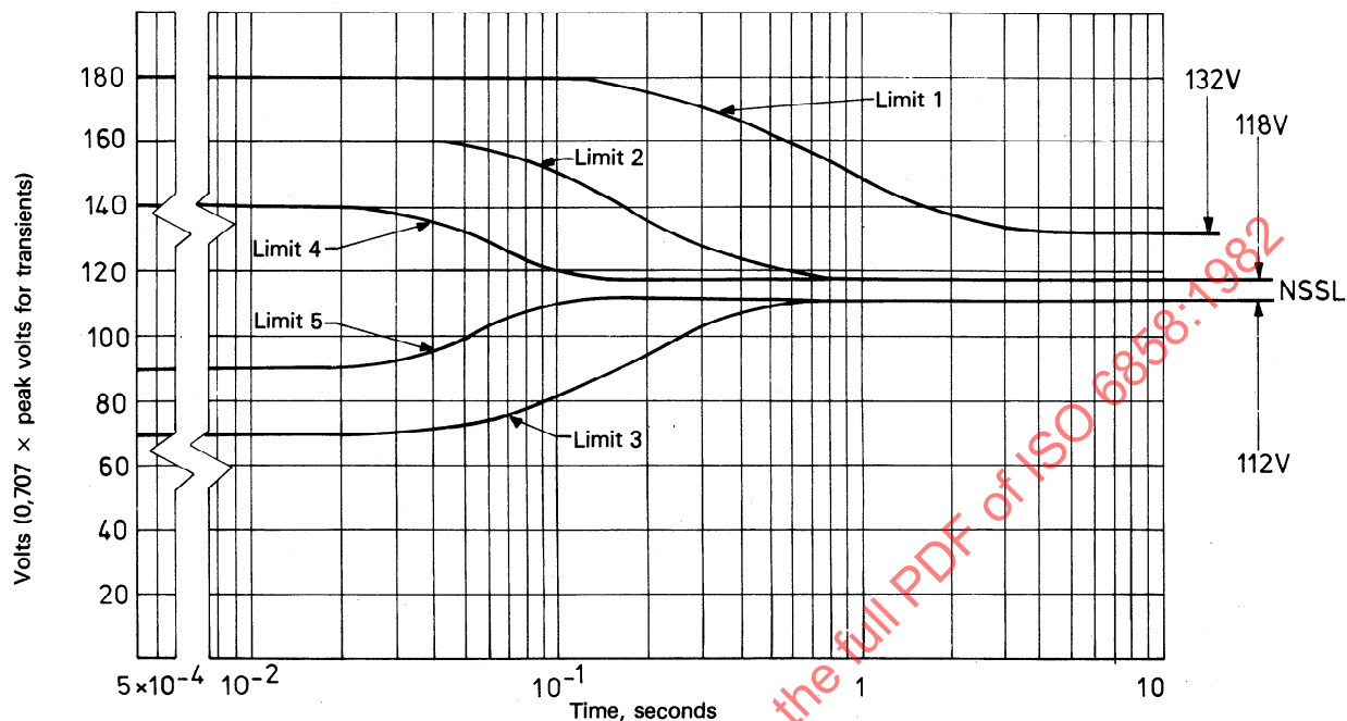
Figure 3 — Envelopes for a.c. surges
