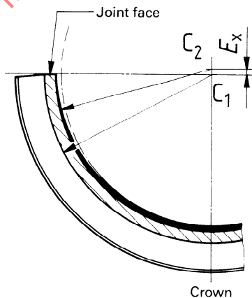
Figure 2 — Eccentric bore
