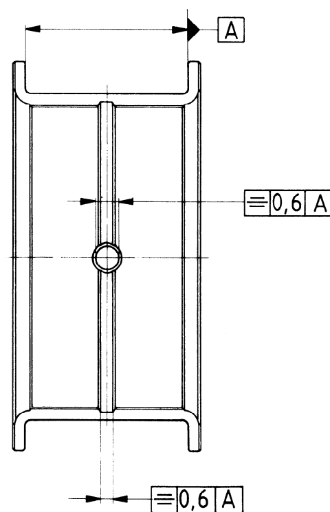
Figure 7 — Position of the annular groove and oil hole in the radial part of the bore
