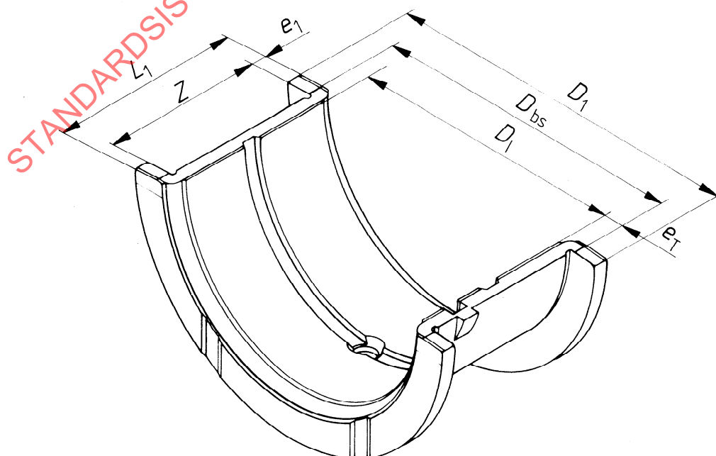
Figure 1 — Flanged half bearing
