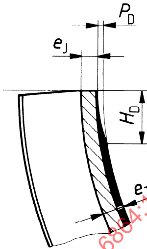
Figure 4 — Joint face bore relief
