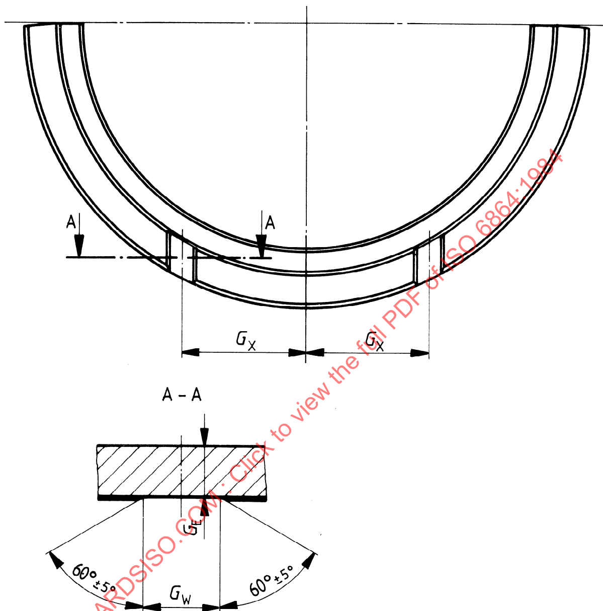
Figure 9 — Groove form on the flange face
