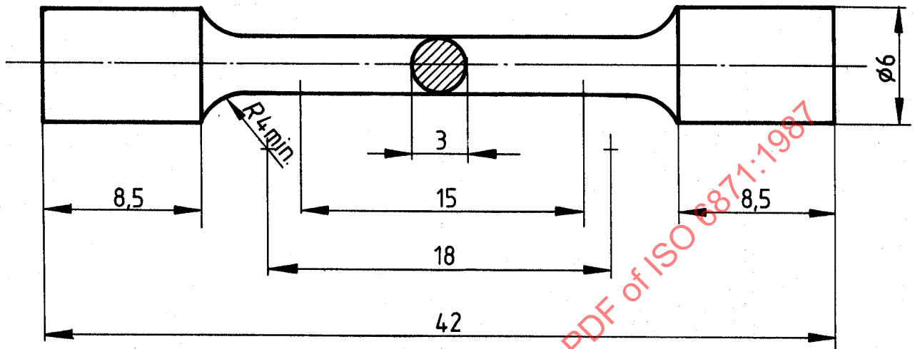
Figure 1 — Tensile test specimen
