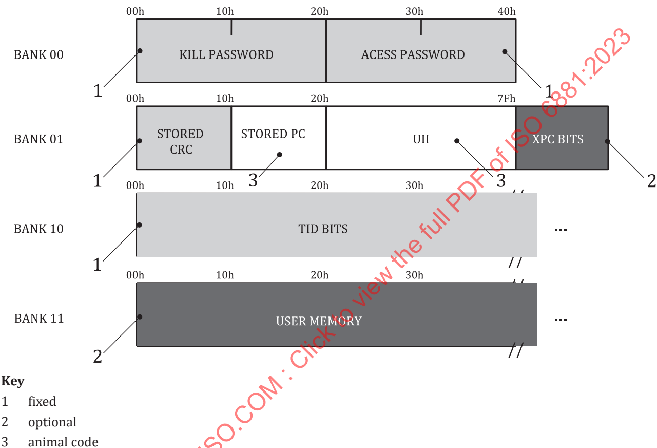
Figure 1 — Memory map of ISO 18000-63 transponder
