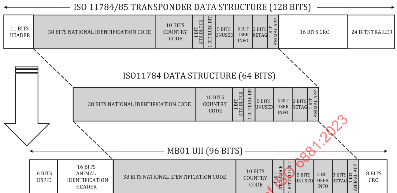
Figure 3 — Backward compatibility with the ISO 11784 scheme
