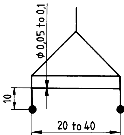
Figure 1 — Stirrup [5.2 a)]
