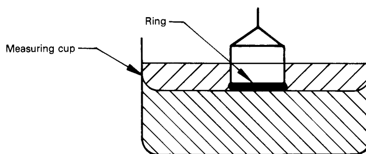
Figure 4 — Ring at "zero position"
