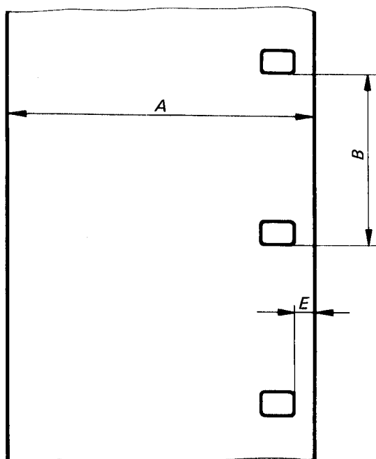
Film with perforations along one edge Type 1 : 16 mm — 1R
