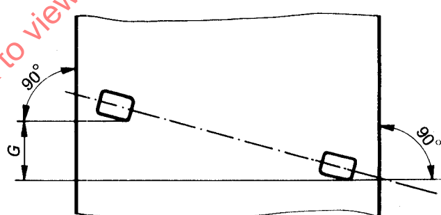
Permissible alignment deviation of the rows of perforations
