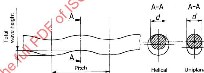
Figure A.2 — Crimps
