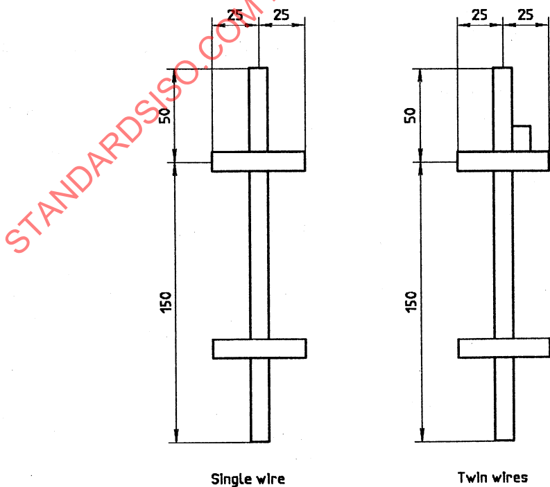
Figure 2 — Test pieces
