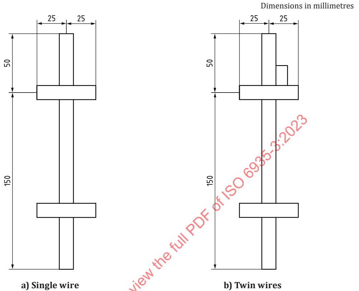
Figure 3 — Test pieces
