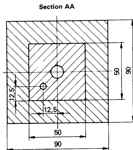
Figure 4 — Receiving calorimeter
