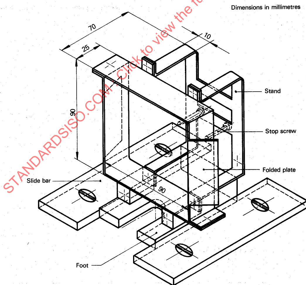
Figure 6 — Calorimeter stand
