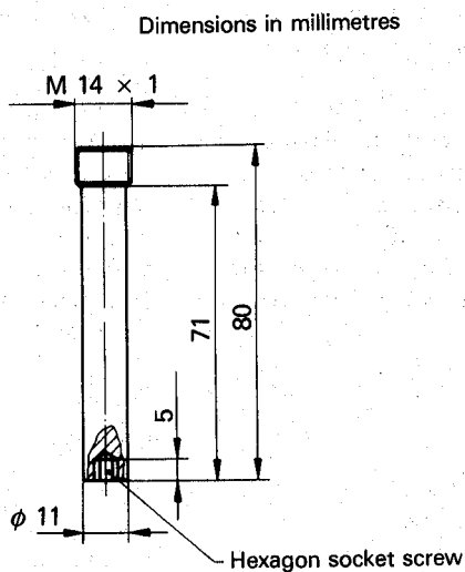
Figure 5 — Heating coil
