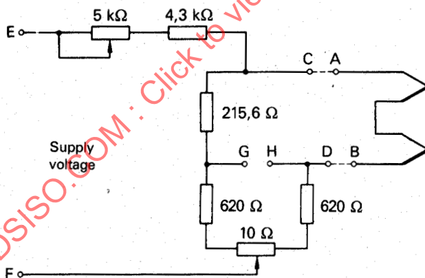
Figure 11 — Diagram of the electrical measuring bridge
