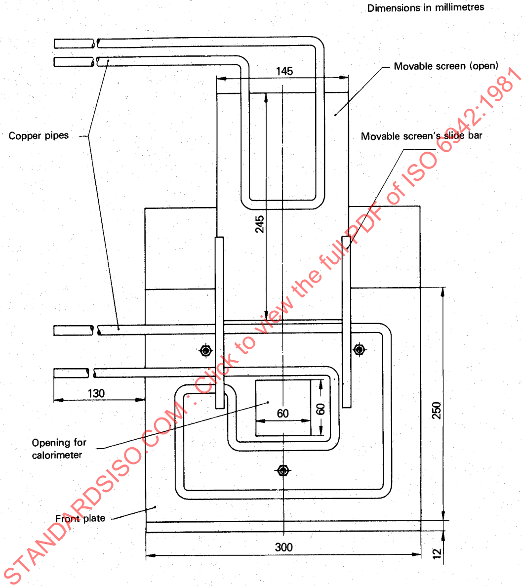
Figure 9 — Cooling system
