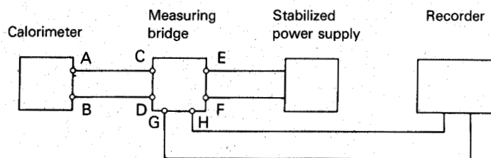
Figure 12 — Arrangement for connection of the parts of the measuring device
