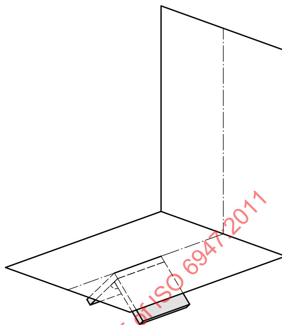
Figure A.20 — Main welding position (PE)
