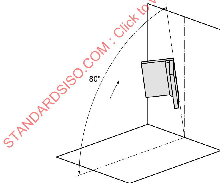
Figure A.21 — Overhead welding position (PE) slope limit
