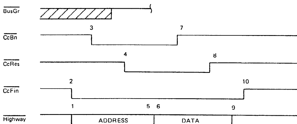
Figure 10. Write cycle
