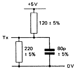
Figure 4. Test circuit
