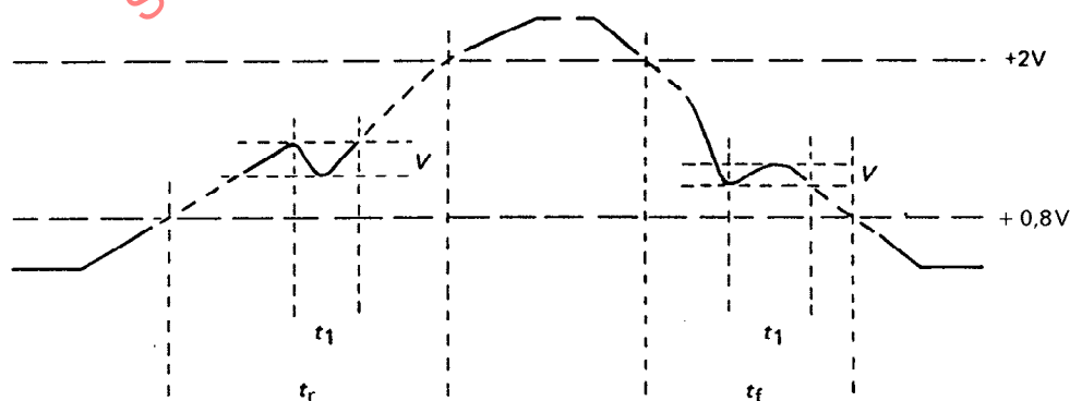
Figure 5. Signal edge characteristics
