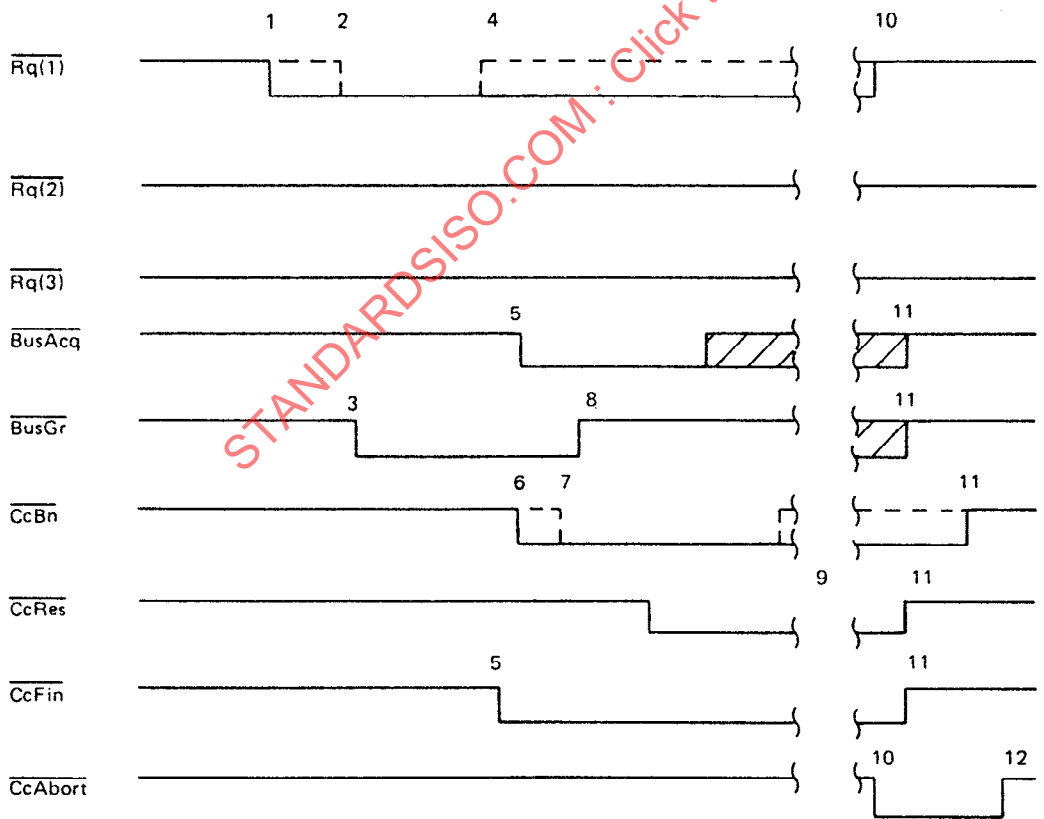
(b) Cycle not allowed by protection device
