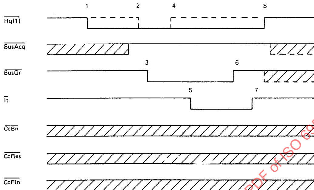
Figure 8. Interrupt cycle
