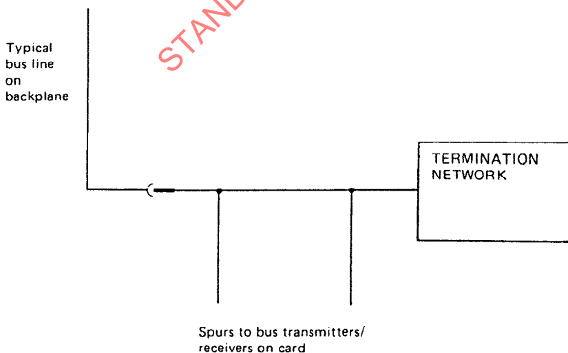
Figure 3. End terminator/spur card
