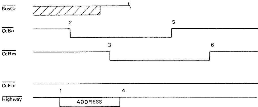
Figure 11. Vector cycle
