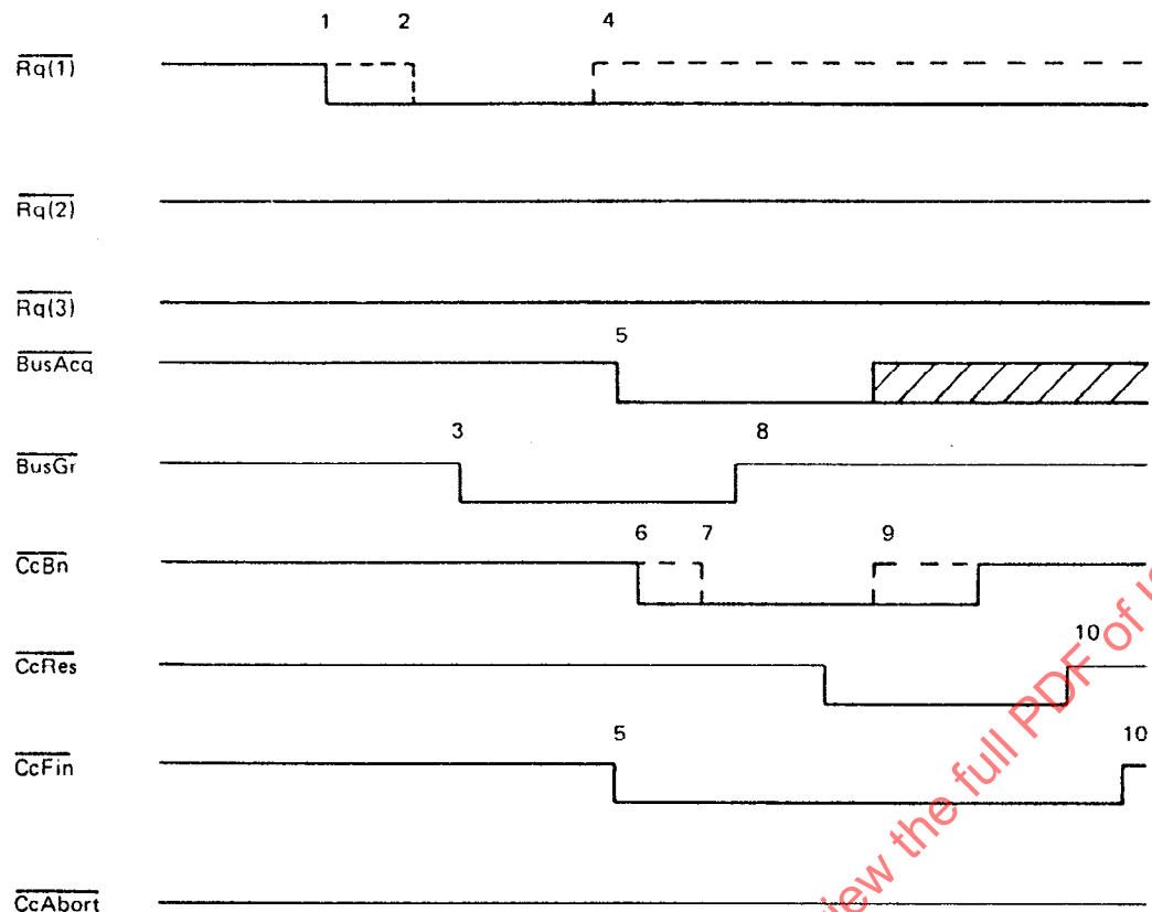
(a) Cycle allowed by protection device
