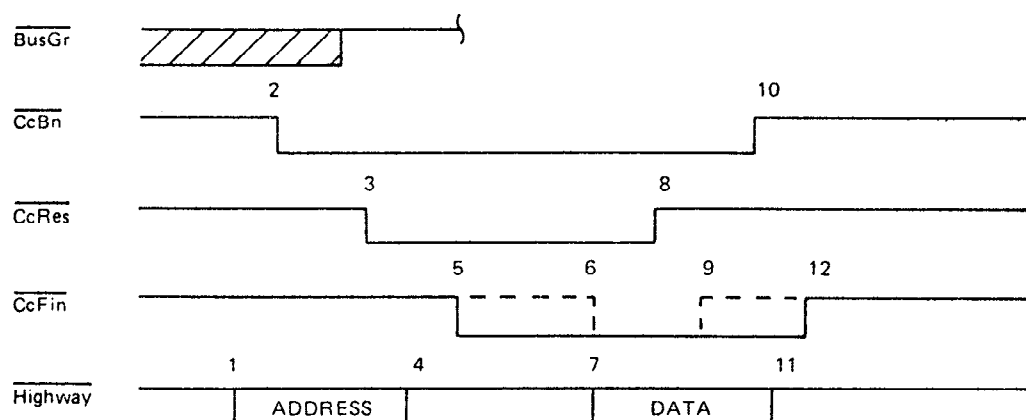
Figure 9. Read cycle
