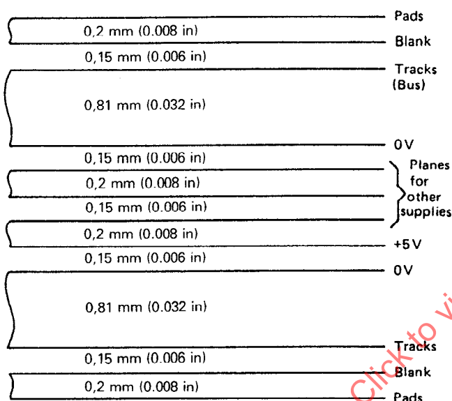
Figure 17. Backplane cross section
