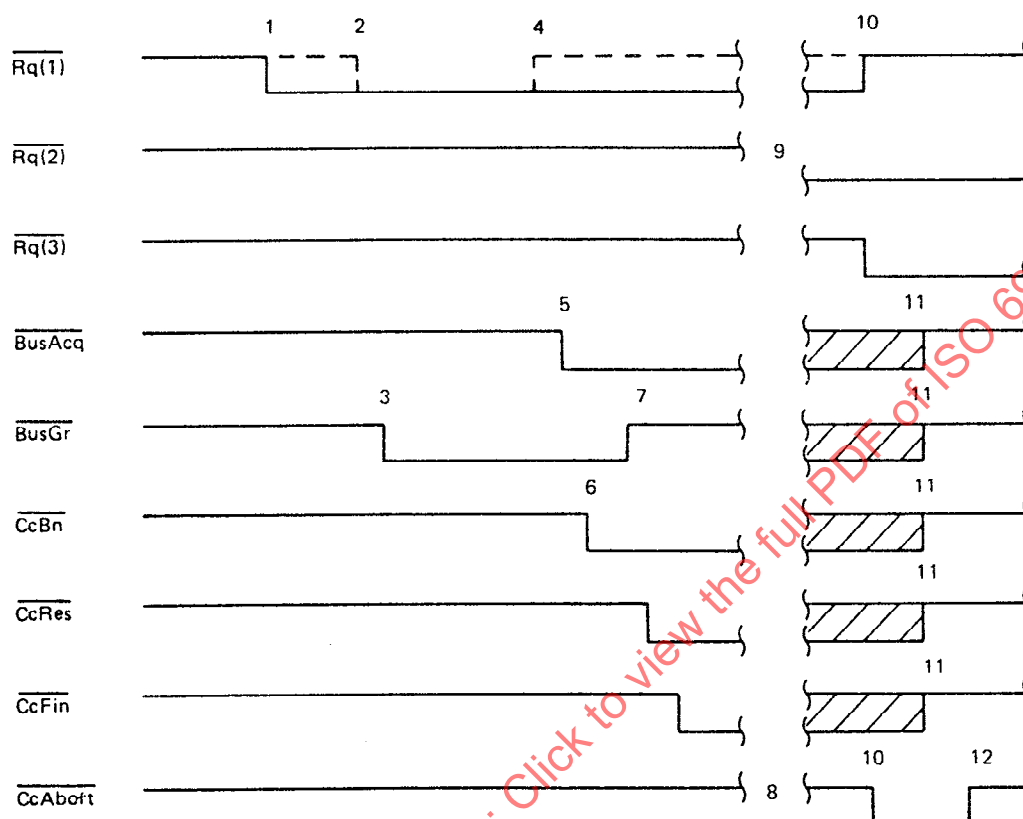
Figure 12. Cycle time-out using cycle abort
