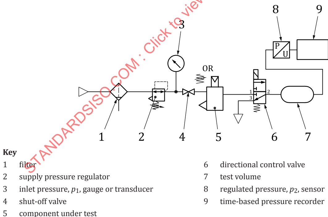
Figure 8 — Typical charging test circuit for repeatability
