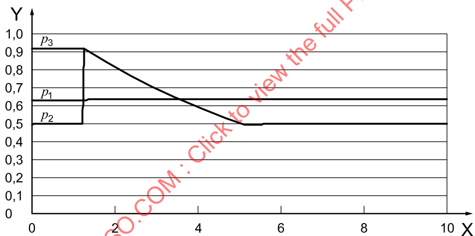
Figure A.6 — Pressure response during charge – component (B)
