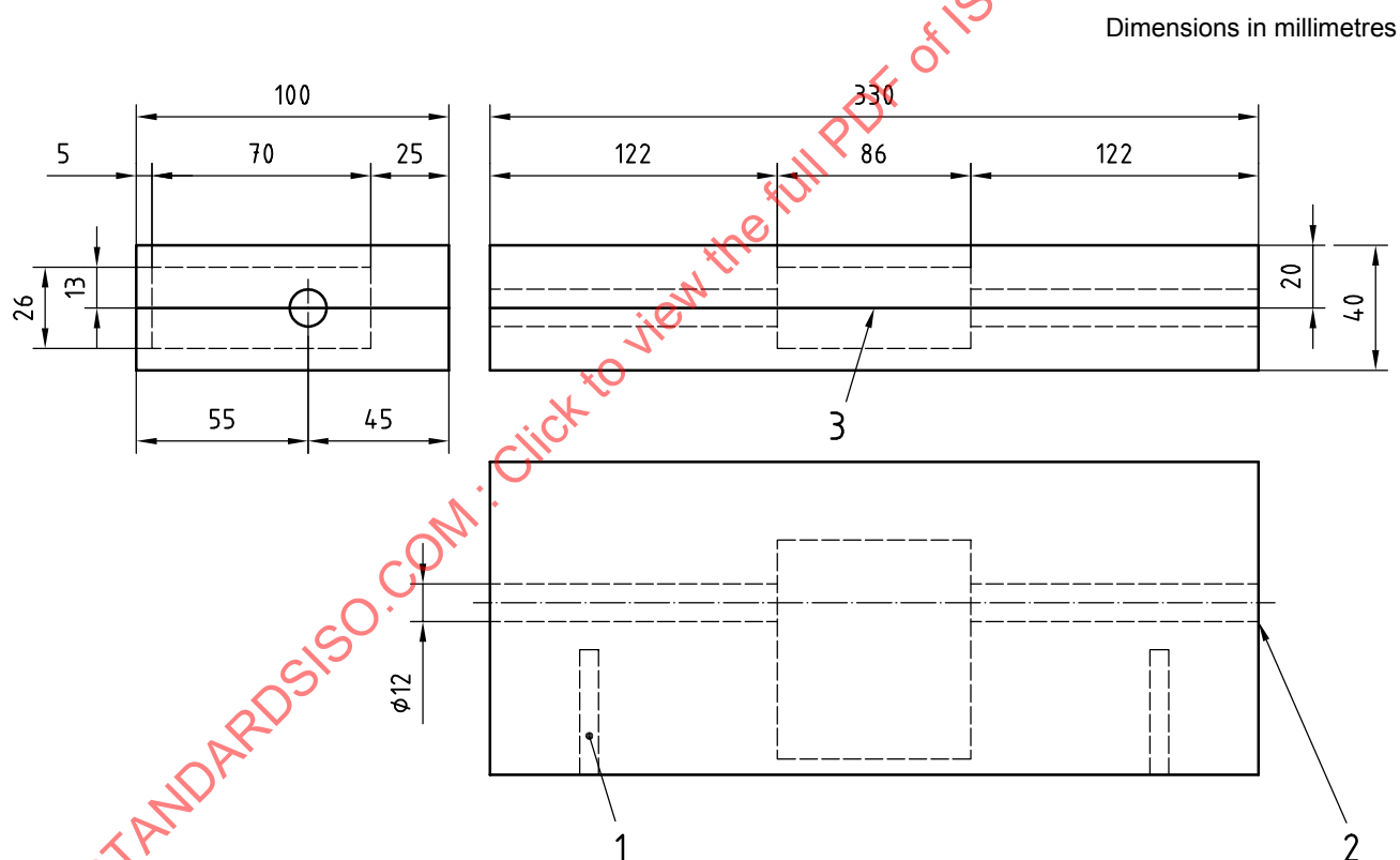
Figure 1 — Sampling apparatus
