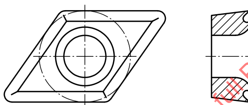
b) DCMT with chip breakers
