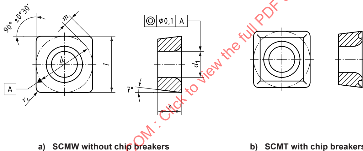
Figure 5 — Square inserts — SC
