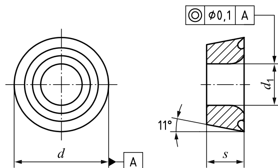
Figure 12 — RPMT with chip breakers
