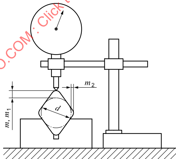
Figure B.3 — Rhombic insert
