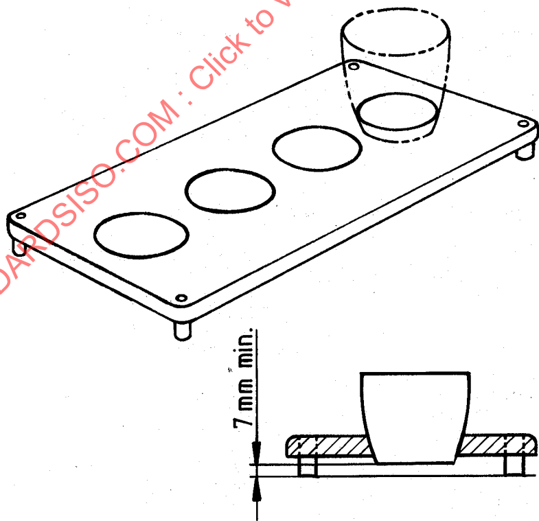
Figure 2 — Support for nickel crucibles
