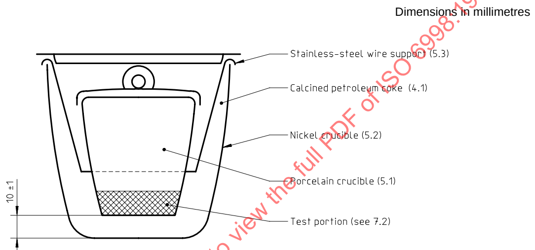
Figure 1 — Nickel and porcelain crucibles assembled together
