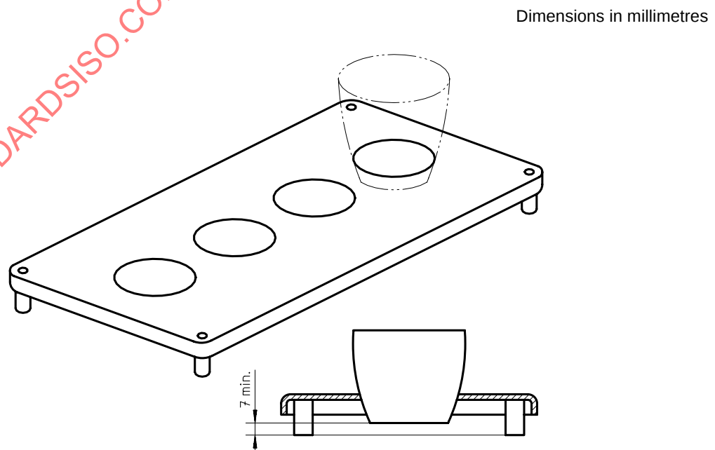
Figure 2 — Rack for nickel crucibles
