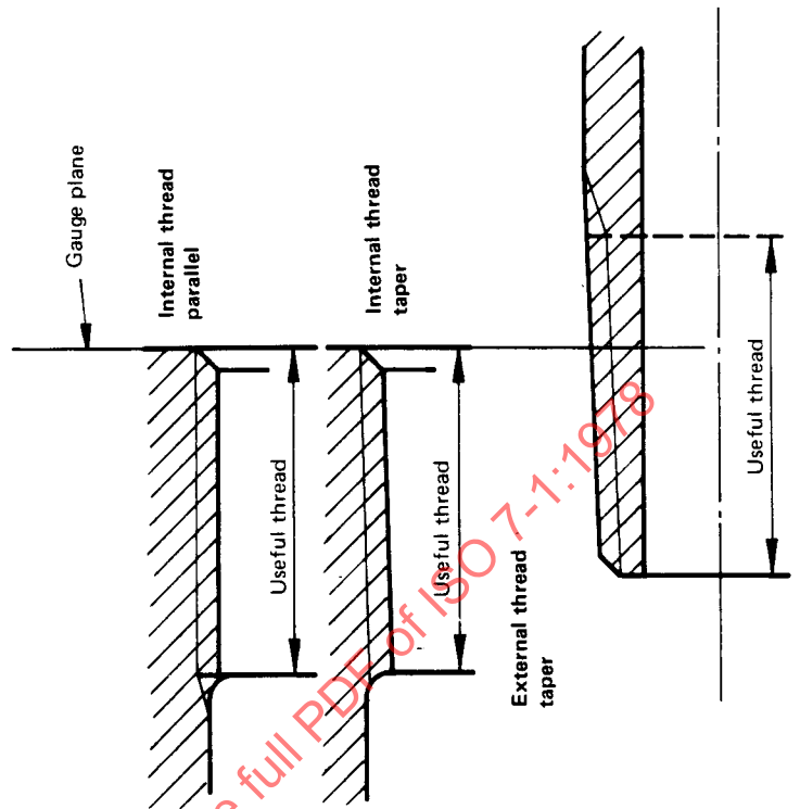
FIGURE 4 — Position of gauge plane, useful thread
