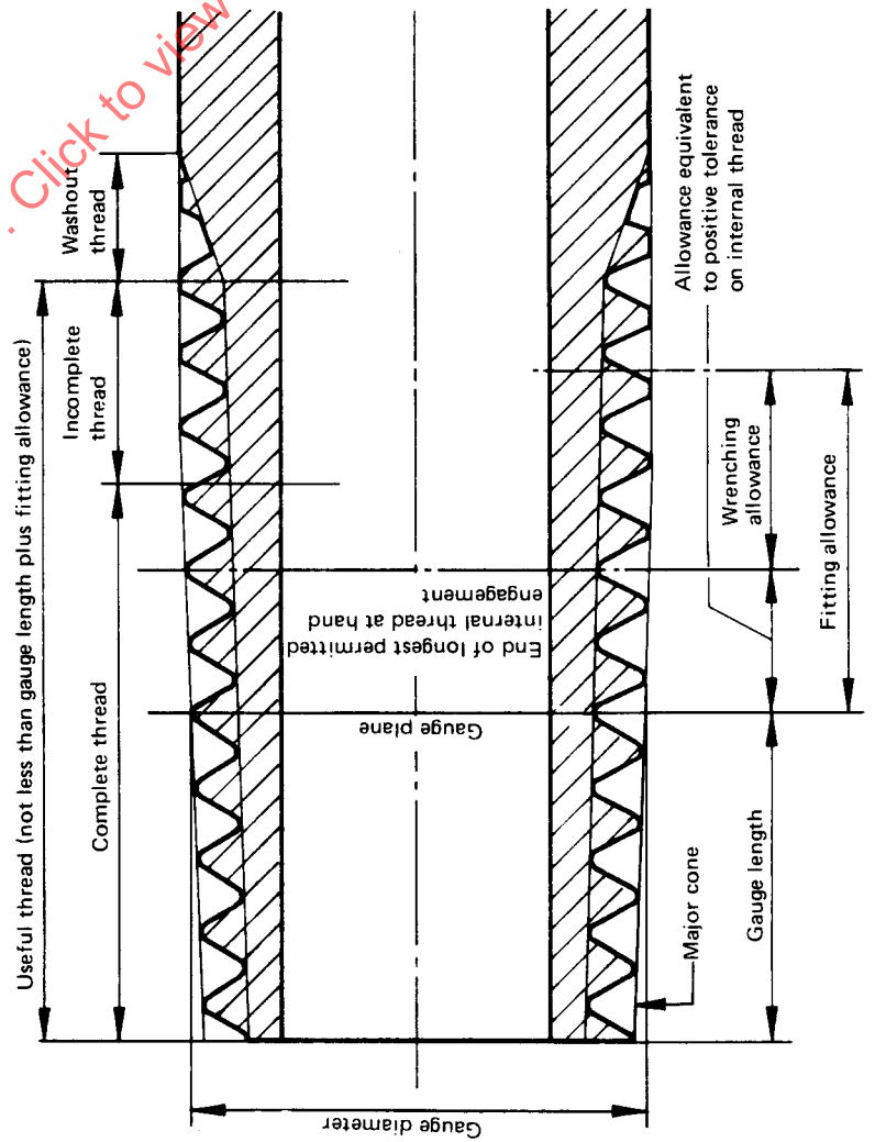
FIGURE 3 — Terms relating to pipe threads
