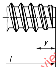
b) Type F (flat end)
