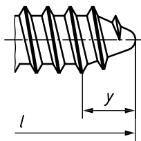
a) Type R (rounded end)
