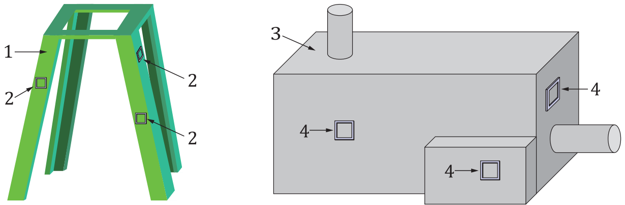
a) Deposition concentration measurement on the steel structure to evaluate the average or median value
