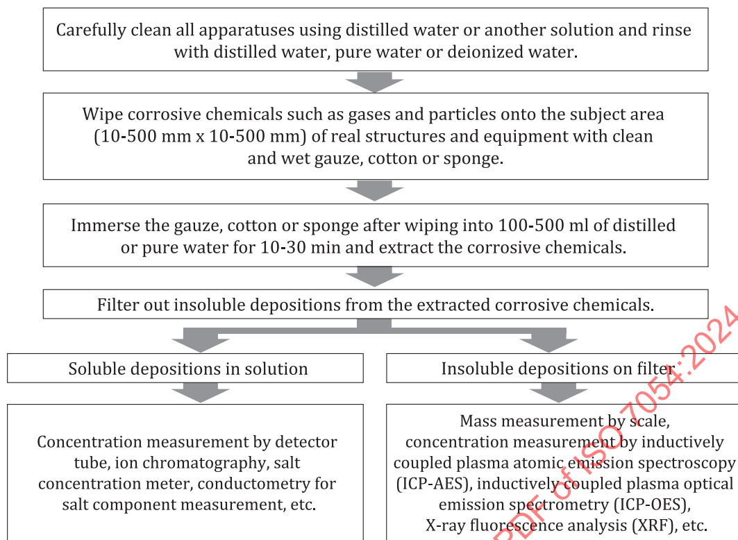
Figure 4 — Flowchart of wiping method
