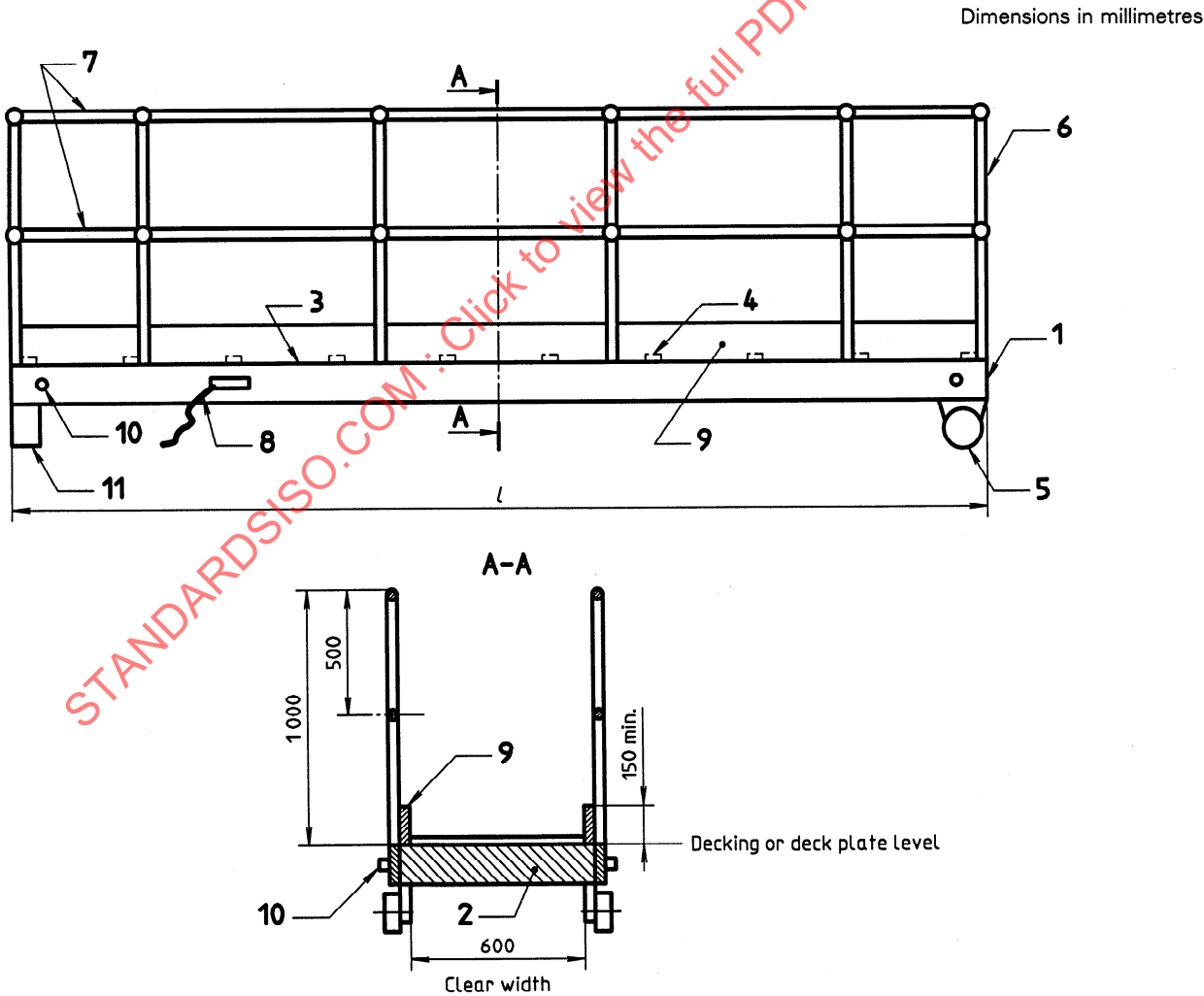
Figure 1 — General arrangement of a gangway (for item numbers, see table 1)
