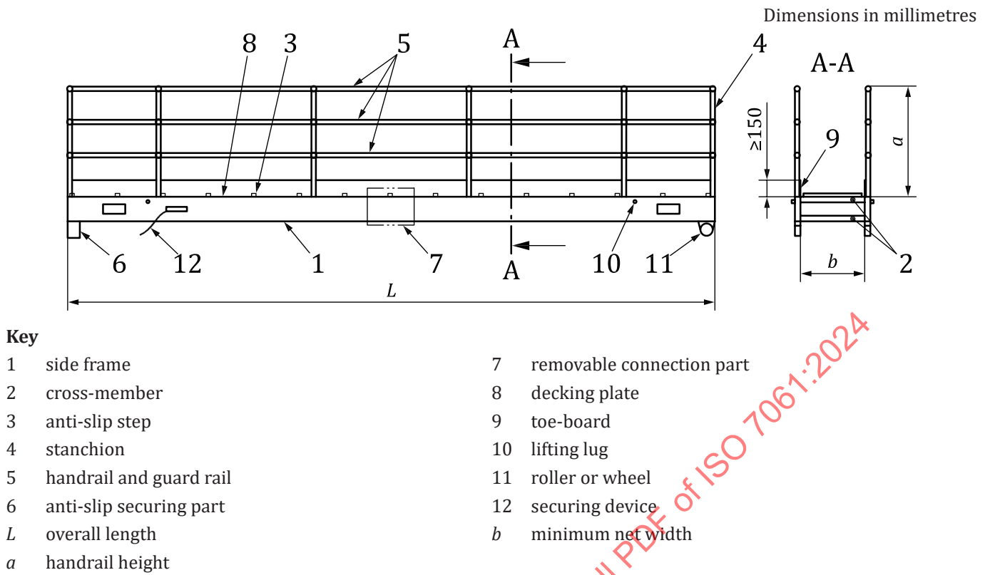
Figure 1 — General arrangement of a Type A gangway
