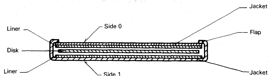
Figure 2 — Section A-A
