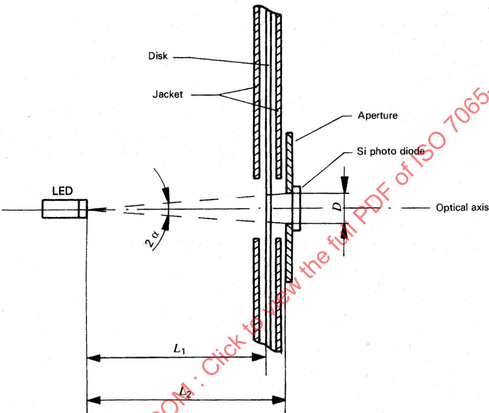
Figure 9 — Measuring device
