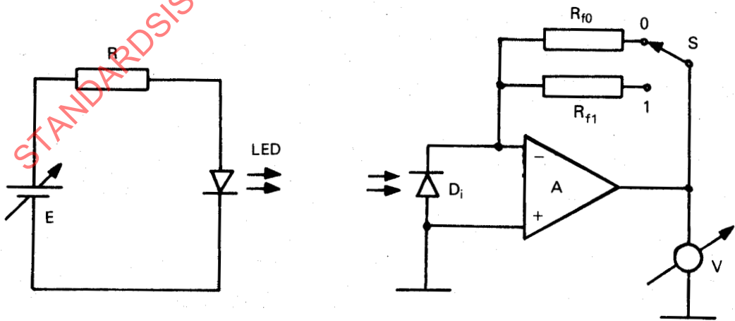
Figure 10 — Electronic circuitry
