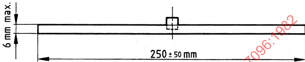
Figure 1 — Design for rigid disc with accelerometer assembly bonded at centre
