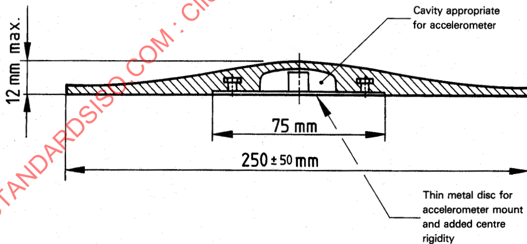
Figure 2 — Design for semi-rigid disc of approximately 80-90 durometer (A-scale) moulded rubber, plastic, etc.
