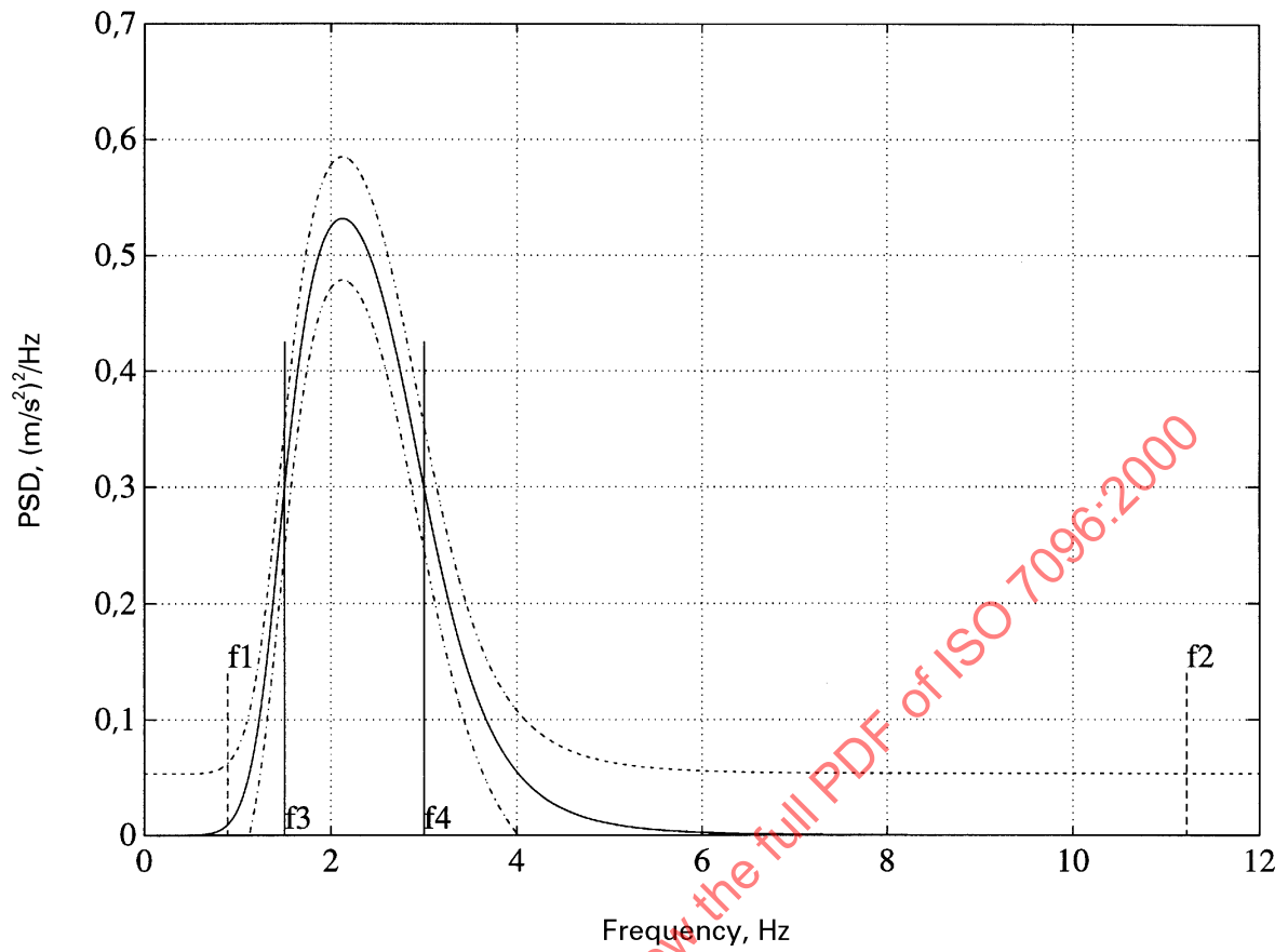
Figure 5 — PSD for input spectral class EM 4 (grader)
