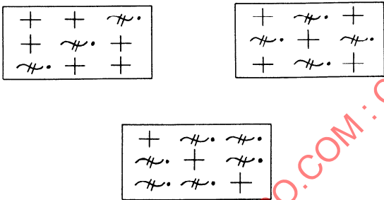
Figure 8 – Charnockite
