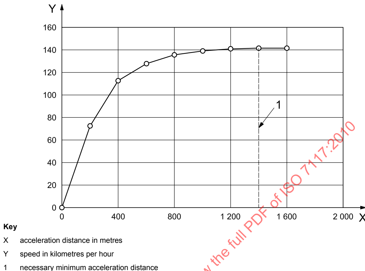
Figure A.2 — Example of relationship between motorcycle speed and acceleration distance in the case of an incremental length of 200 m
