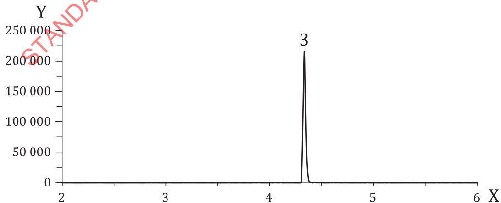
b) Fipronil-desulfinyl
