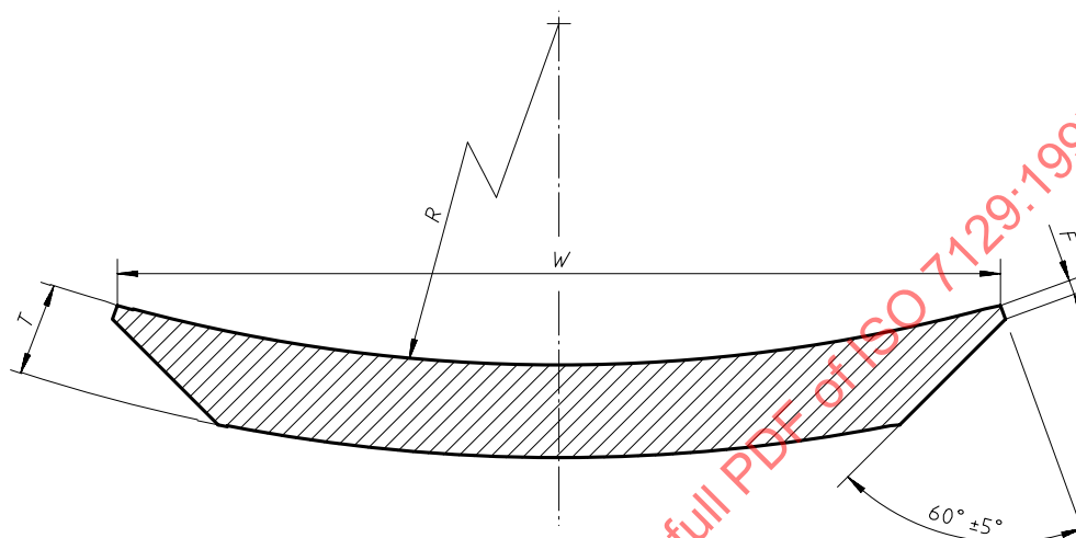
Figure A.2 — Cutting edge for graders
