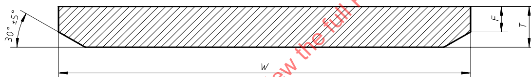
Figure 1 — Cutting edge for tractor-dozers and scrapers
