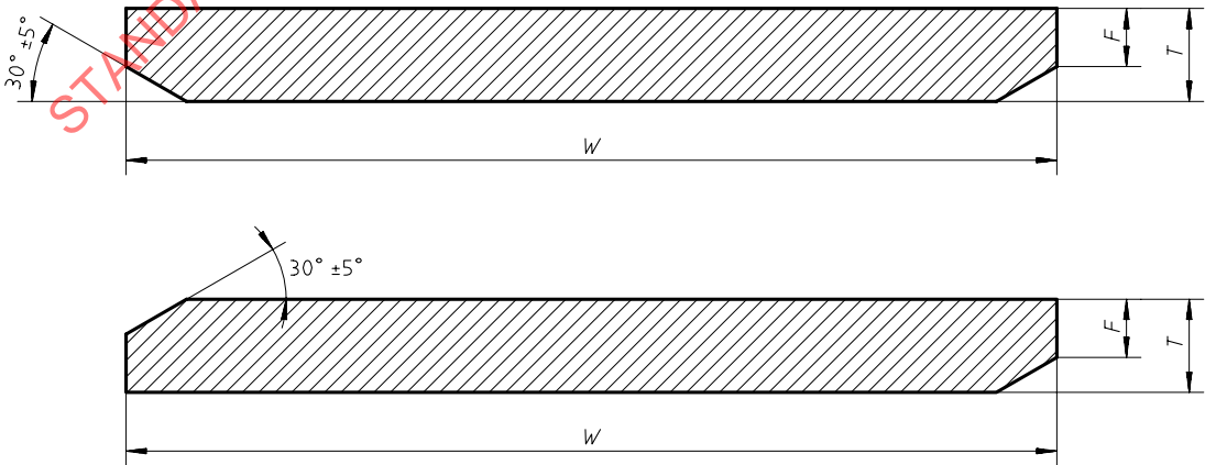
Figure A.1 — Cutting edge for tractor-dozers and scrapers
