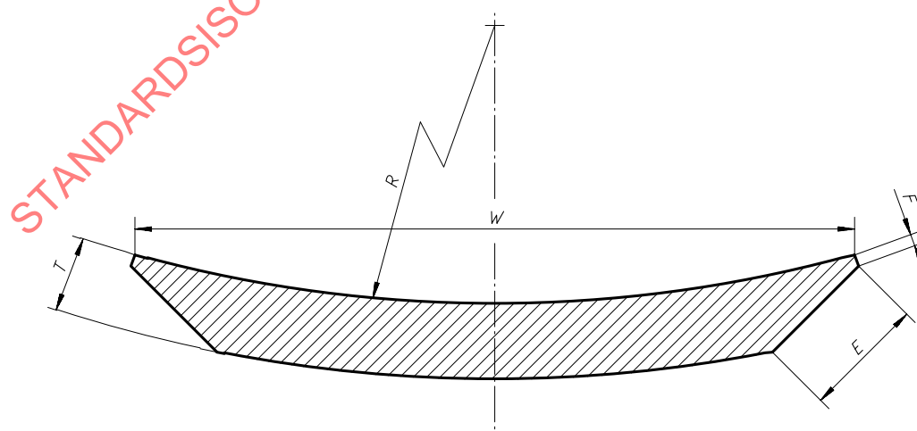
Figure 2 — Cutting edge for graders
