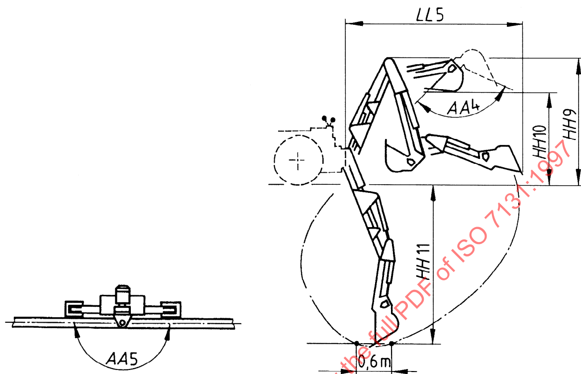
Figure 18 — Dimensions of backhoe
