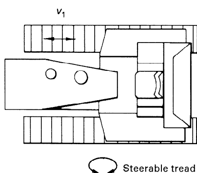
Figure 10 — Crawler skid steer
