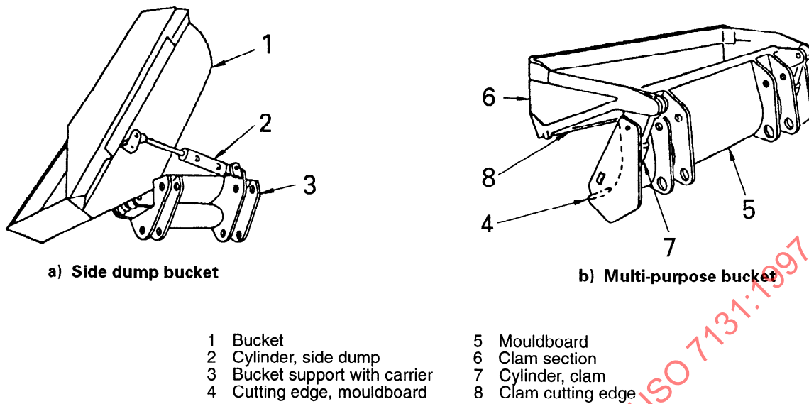
Figure 25 — Nomenclature for attachments
