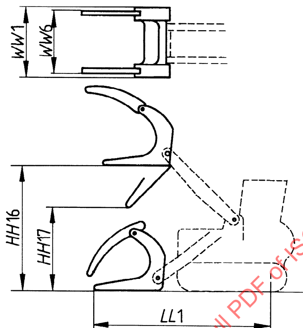
Figure 23 — Dimensions of log fork (log grapple)
