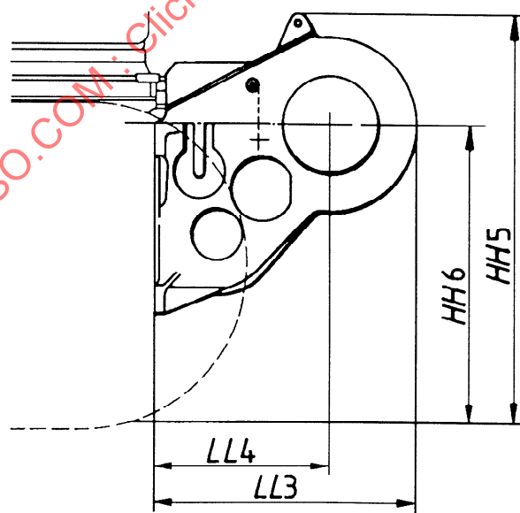
Figure 24 — Dimensions of winch
