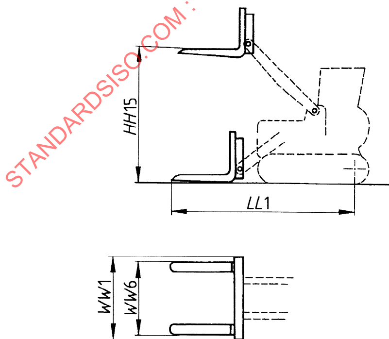
Figure 22 — Dimensions of pallet fork
