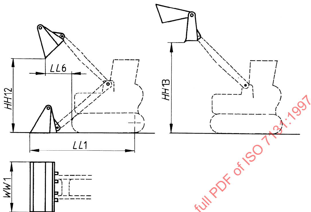
Figure 21 — Dimensions of multi-purpose bucket
