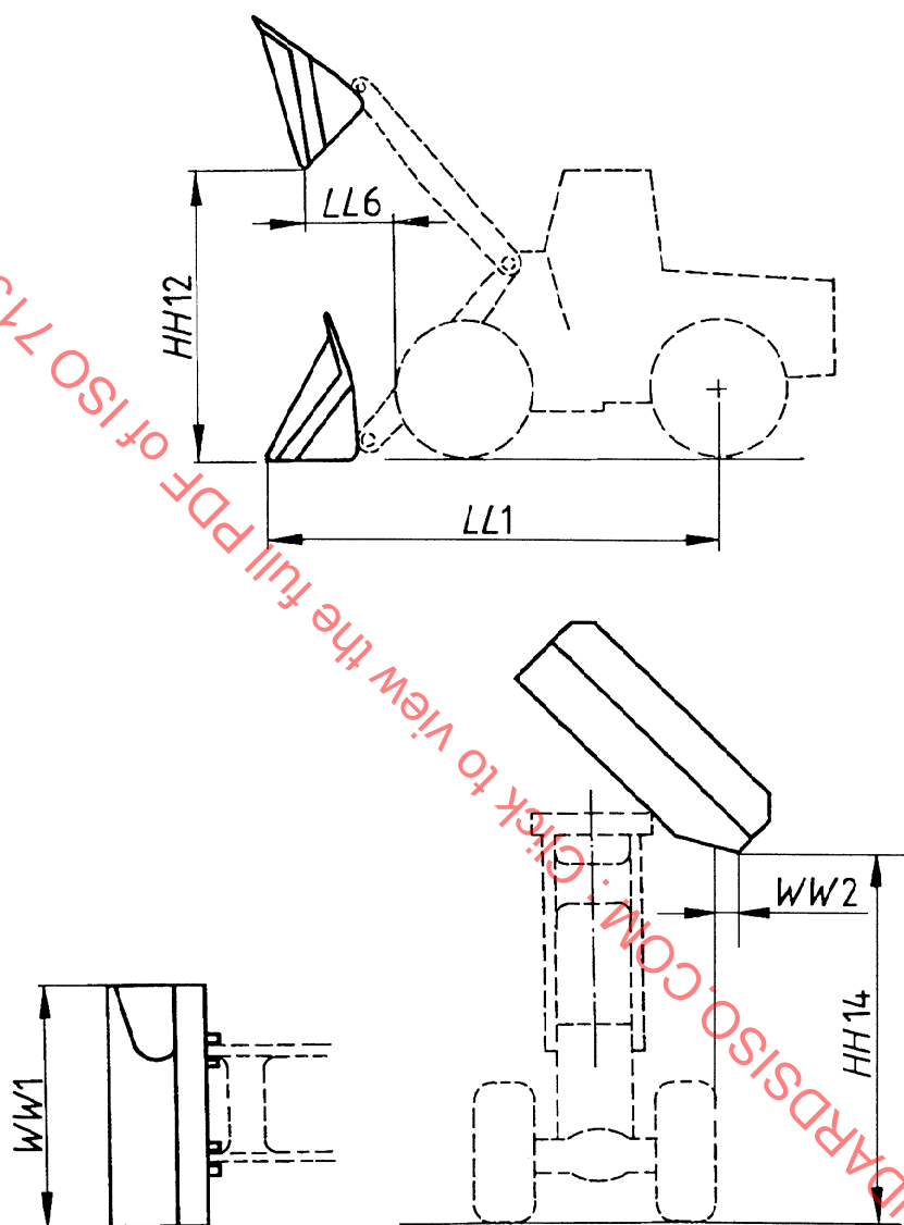
Figure 20 — Dimensions of side dump bucket
