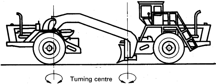
Figure 11 — Double articulated frame steer grader
