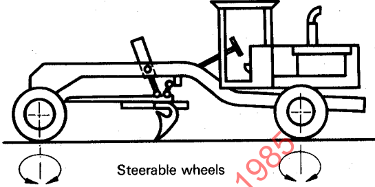
Figure 8 — Front wheel and rear wheel steer grader
