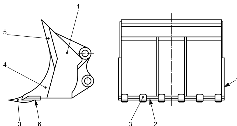
Figure 19 — Shovel bucket
