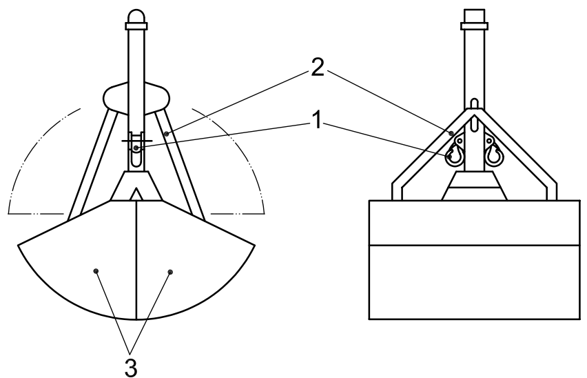
Figure 16 — Clamshell bucket
