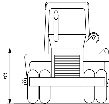
Figure 9 — Dimension H3 for wheeled machine
