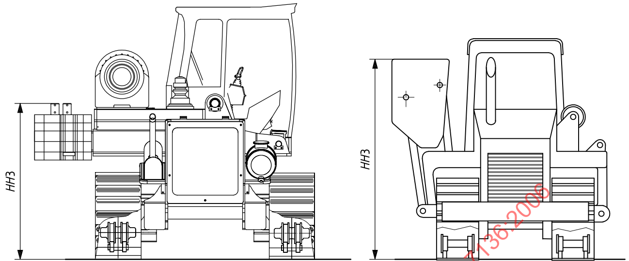
Figure 11 — Dimension HH3
