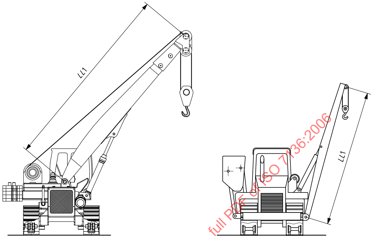
Figure 7 — Dimension LL1
