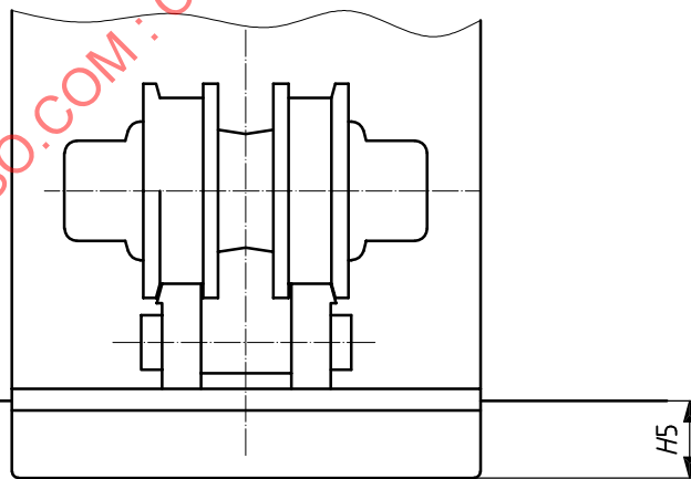
Figure 10 — Dimension H5
