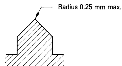
Figure 1 — Fulcrum
