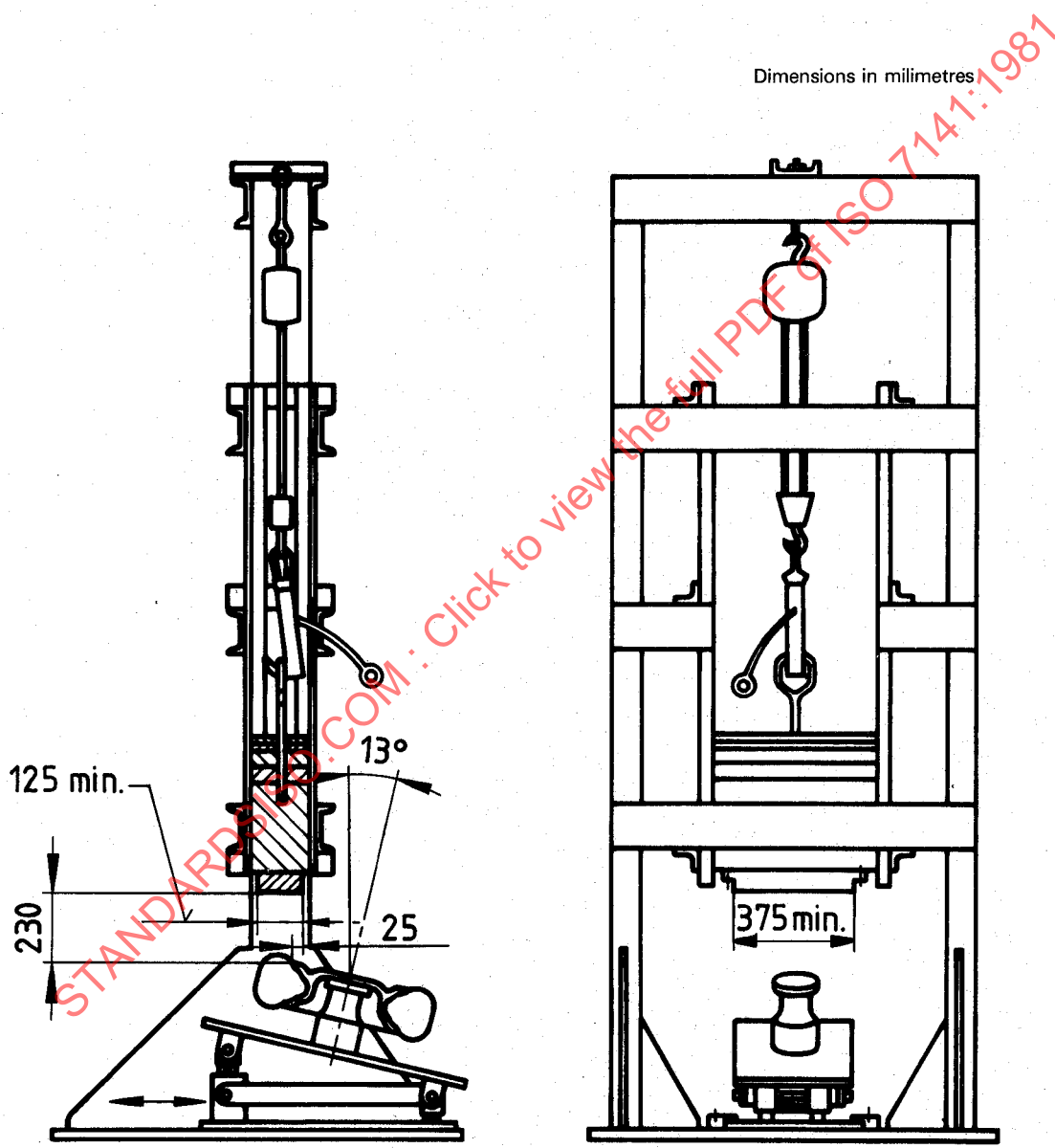
Figure 1 — Impact loading test machine
