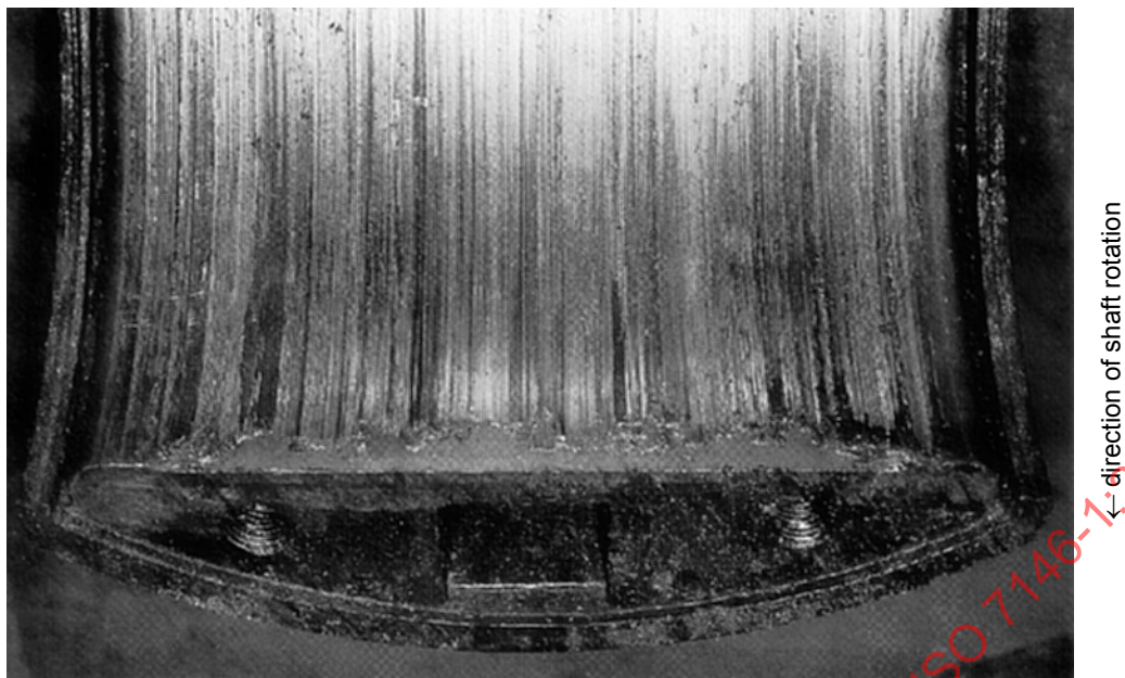
Figure 32 — Cement mill bearing with contamination by cement particles entrained by the oil as a result of damaged seals. Particle-migration tracks are visible (material: steel/tin-based white metal)
