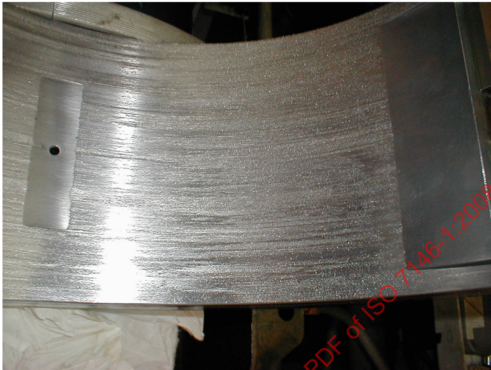
Figure 46 — Formation of electric arc craters
