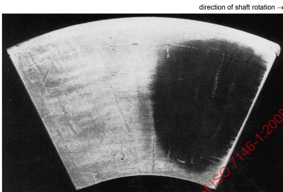
Figure 19 — Thrust bearing tilting pad with deposits of oil carbon (material: steel/tin-based white metal)
