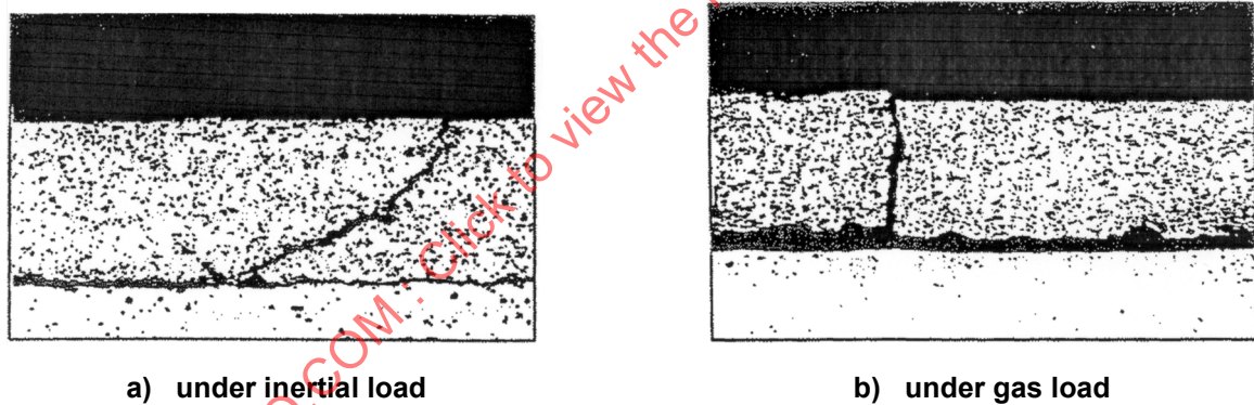
Figure 6 — Typical fatigue cracks of internal combustion engine bearing (material: steel/aluminium alloy)
