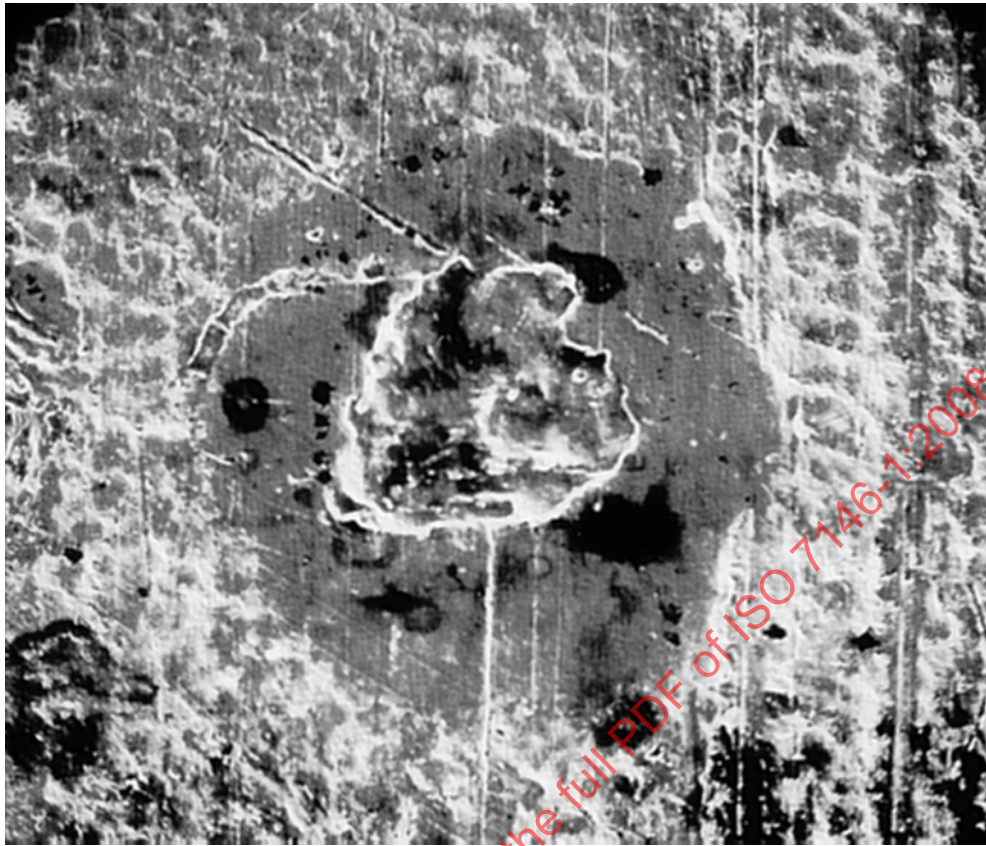
Figure 30 — Crater left by displaced particle surrounded by reflective ring (halo), characteristic of embedding, see Figure 28, label 6, (material: steel/lead bronze/electroplated overlay)
