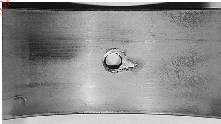
Figure 4 — Flow cavitation erosion at the oil hole of a rod half big-end bearing in a petrol engine (material: steel/Al-Sn)
