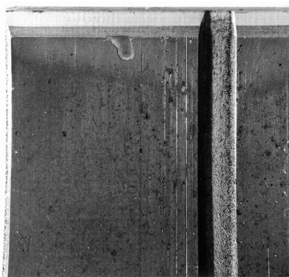
Figure 7 — Flow cavitation erosion at the joint face relief in a big-end bearing
