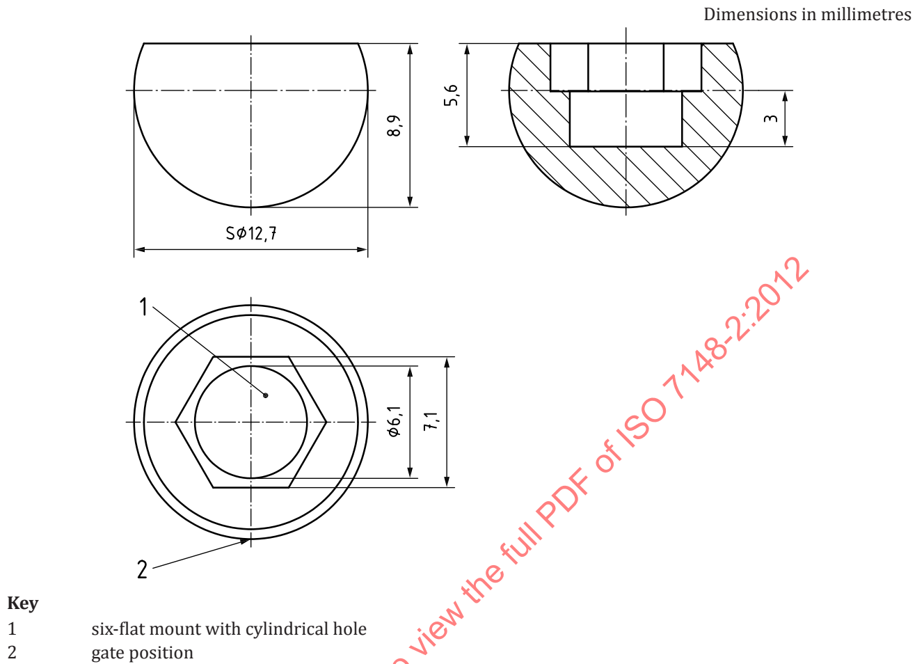
Figure 8 — Example of an injection-moulded sphere
