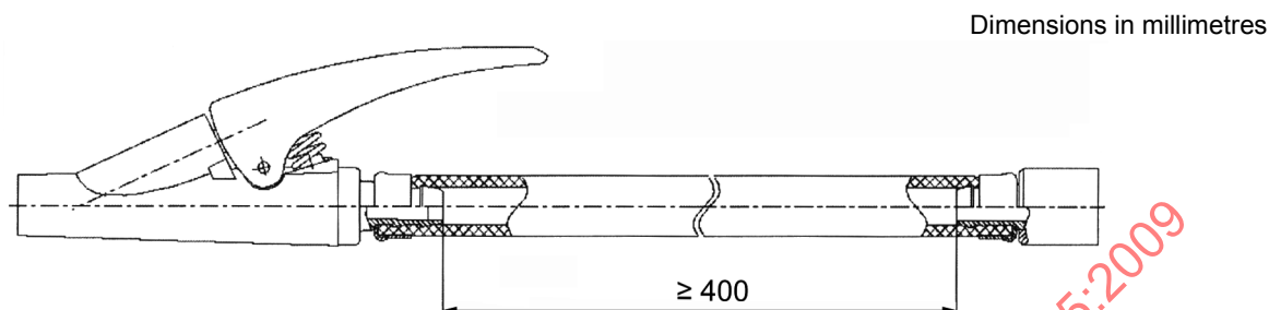
Figure 8 — Minimum hose length
