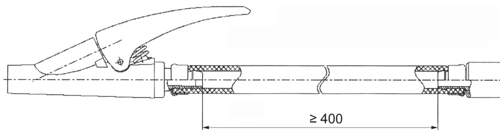
Figure 8 — Minimum hose length
