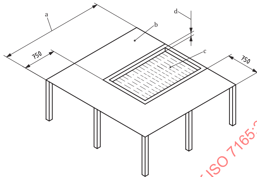
a) Ratings 15F, 25F and 75F (Type B)
